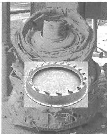
Figure 43: The engine found in Murray Street near the World Trade Center. Does the 'Tobiduct' prove that the 'Flight 175' engine did not come from a standard 767? Some say yes, but others challenge that.
